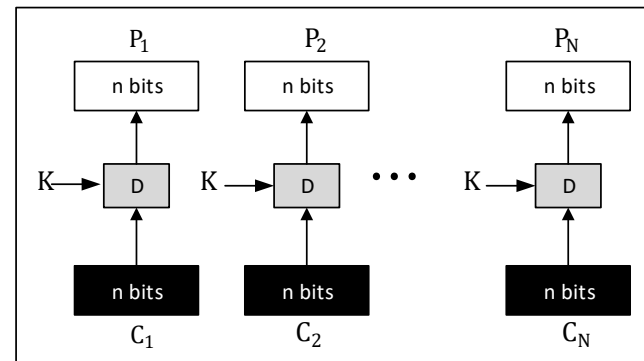
Decryption
