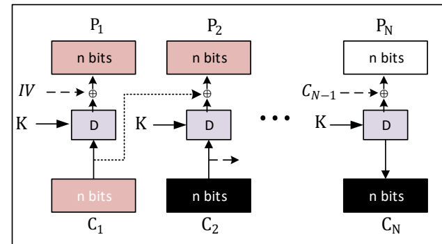
Encryption
