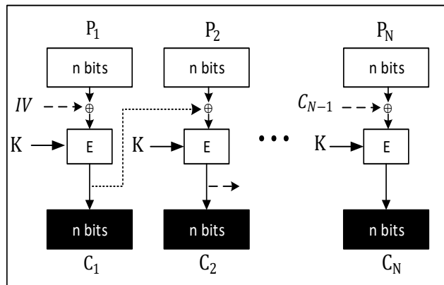
Encryption
